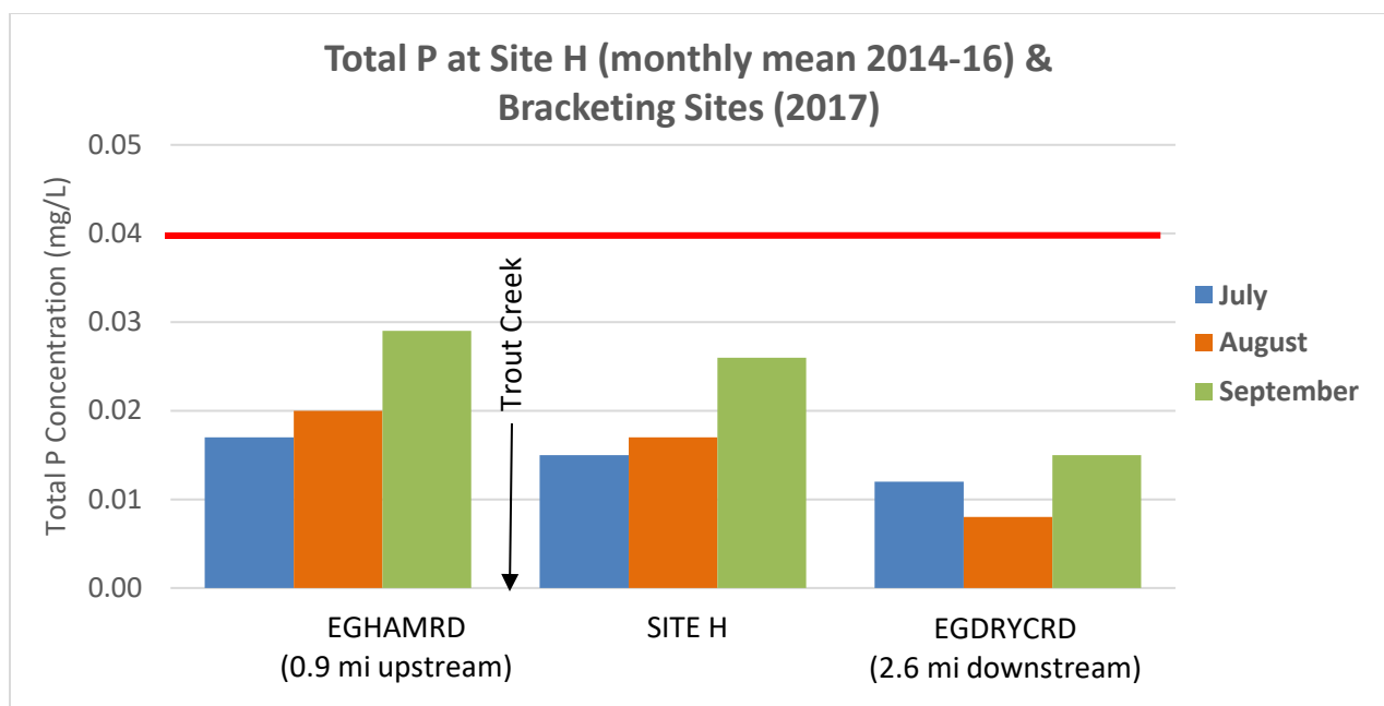
Figure 6. Monthly total phosphorus concentrations for July – September are shown for Site H and the 2017 sites bracketing it. The reach-specific DEQ numeric nutrient criteria (0.04 mg/L) is shown in red. Trout Creek enters the East Gallatin River between EGHAMRD and Site H.
